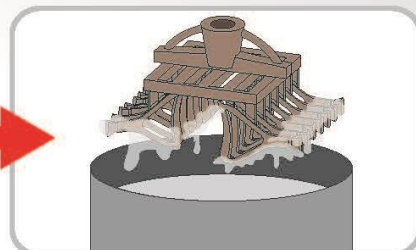
4. Dipping
