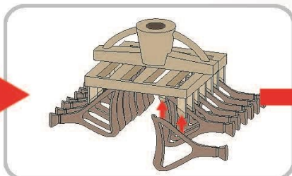
3. Wax pattern assembly
